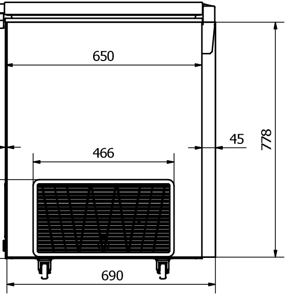
LEFT SIDE: Sticker 690 x 778 mm
