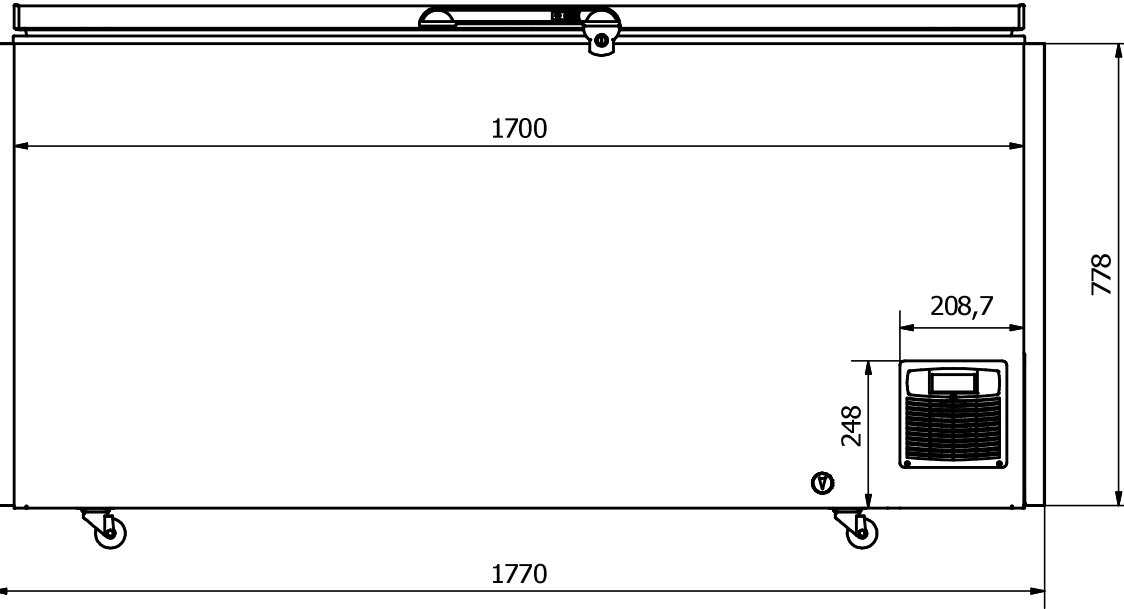
FRONT: Sticker 1770 x 778 mm
